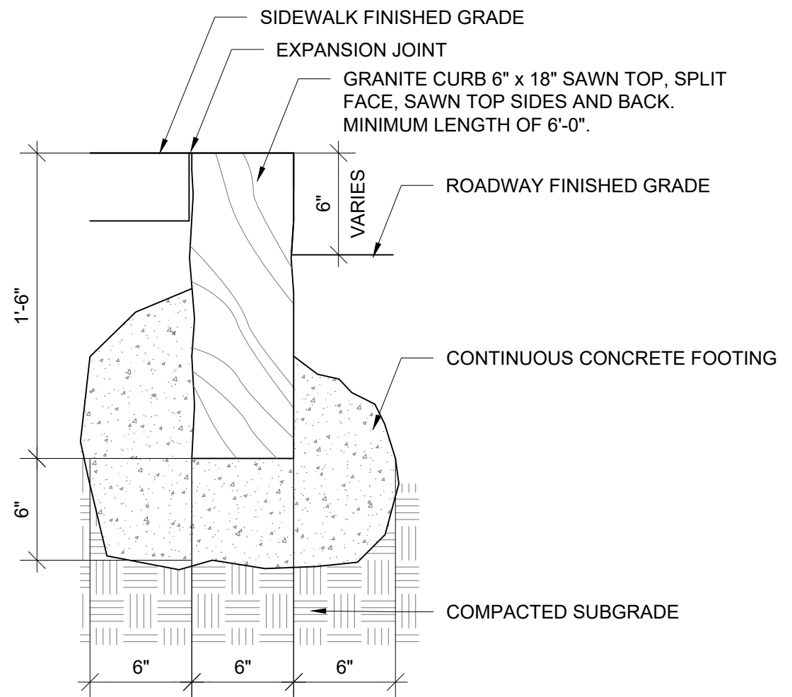
GRANITE STREET CURB: SECTION
