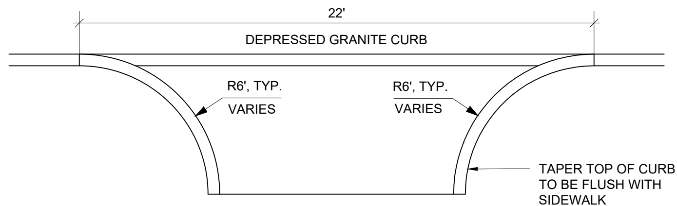
DEPRESSED GRANITE CURB AT DRIVE APRONS: PLAN
