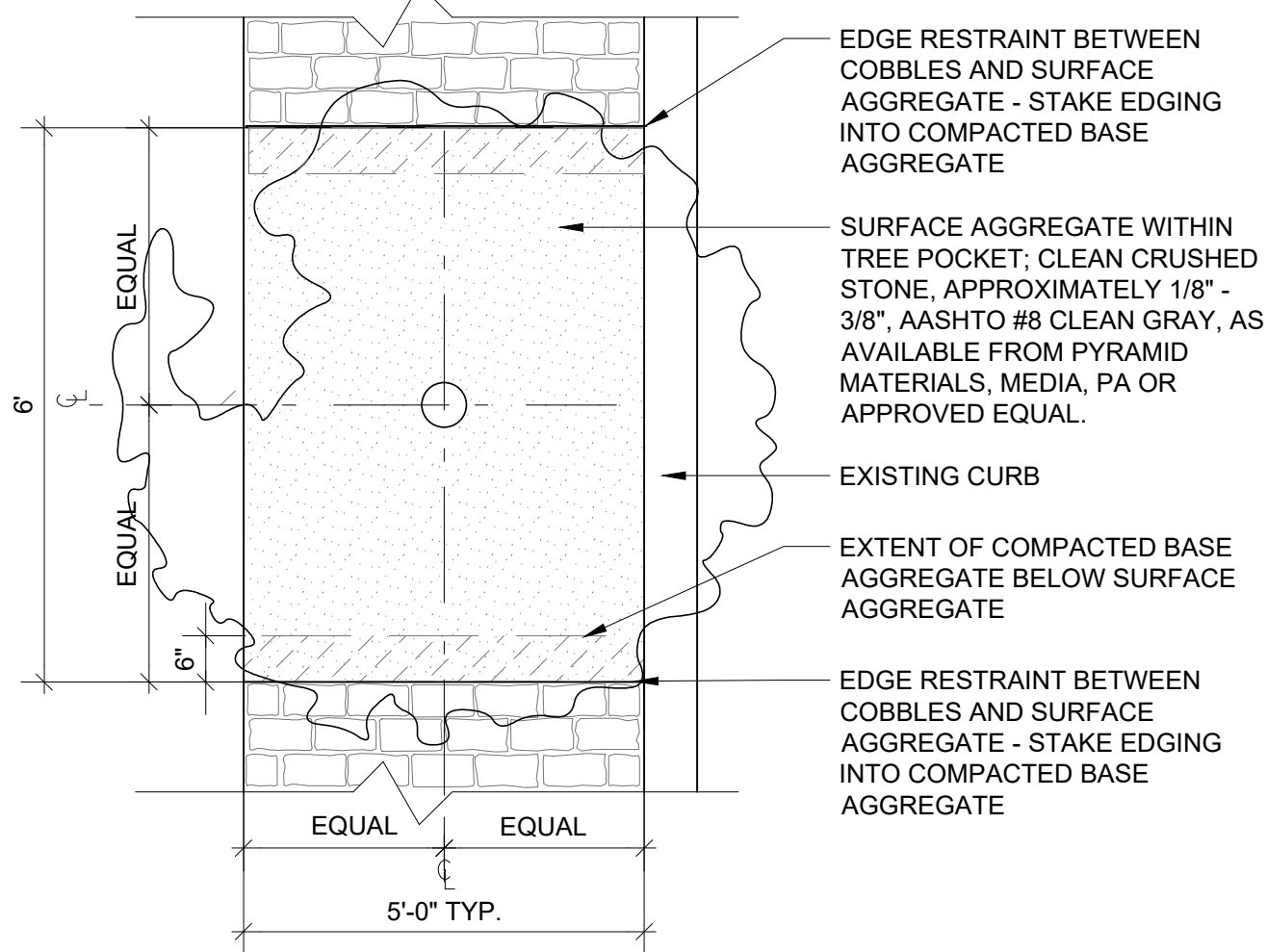
STREETSCAPE: PLAN
