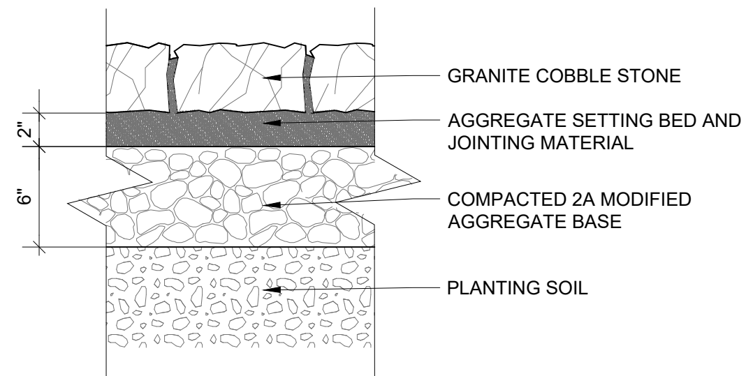
GRANITE COBBLES: SECTION
