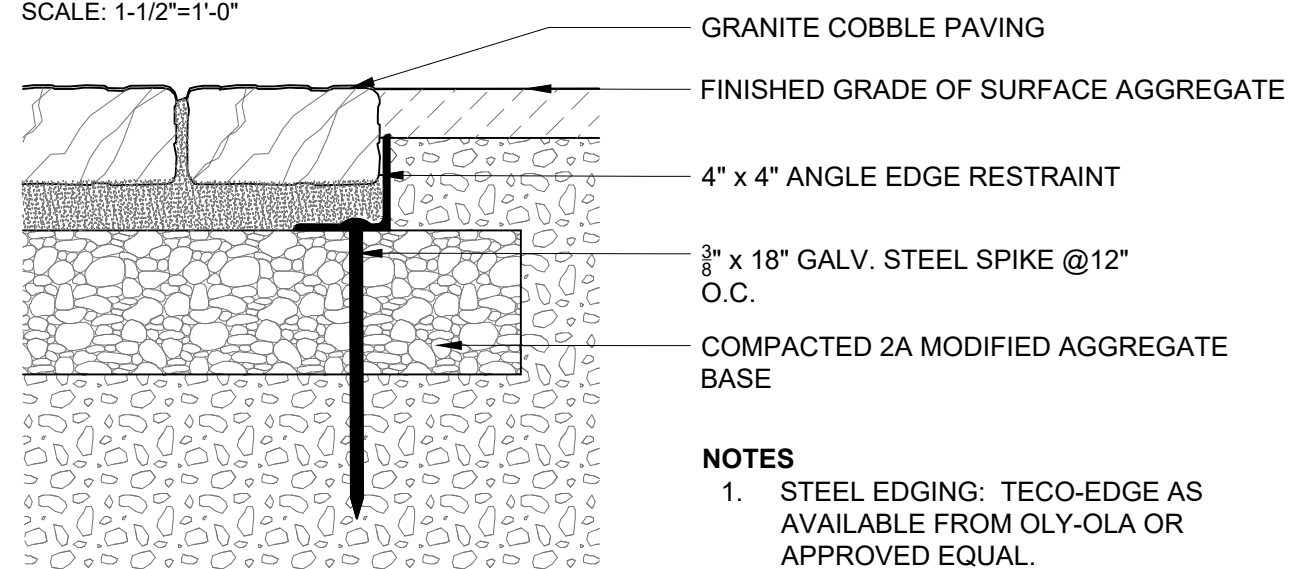
STEEL EDGING: SECTION
