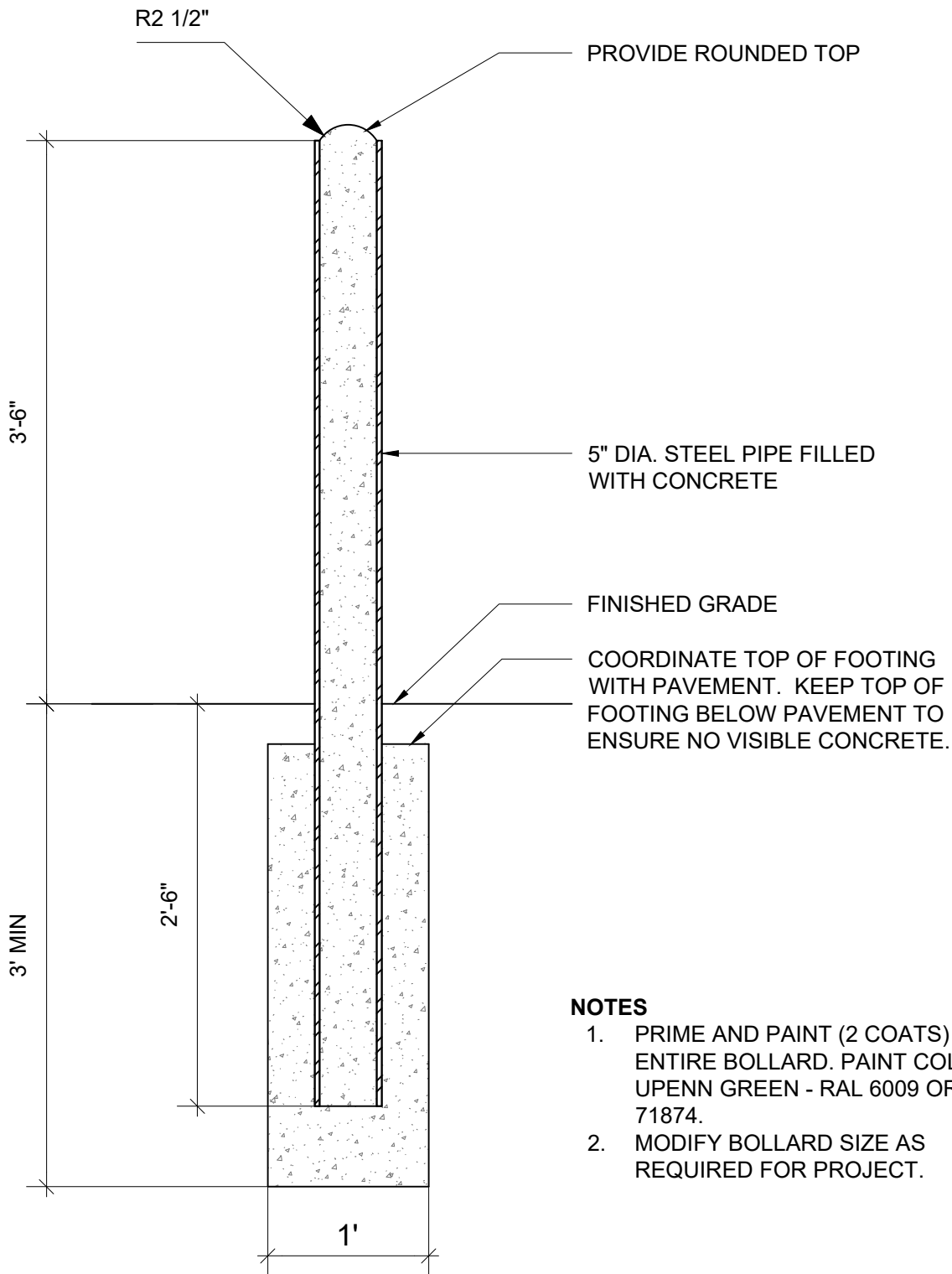
BOLLARD - UTILITY: SECTION
