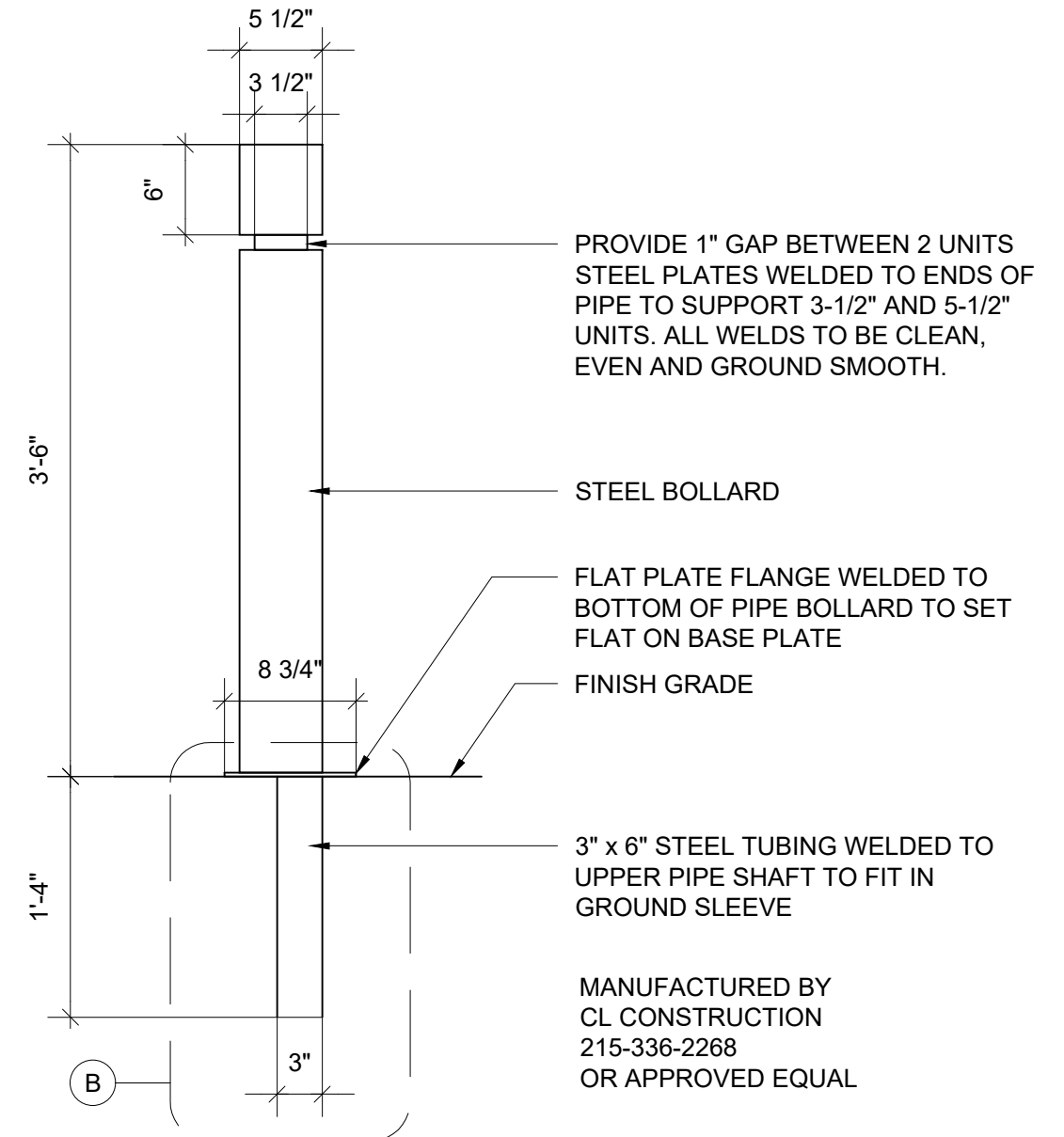
PAINTED BOLLARD - REMOVABLE: SECTION - A
