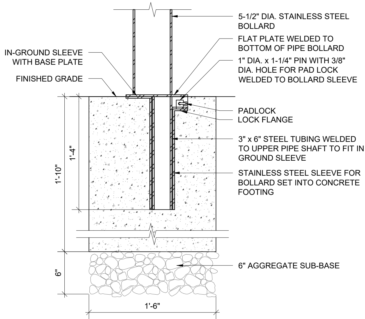
PAINTED BOLLARD - REMOVABLE: SECTION - B
