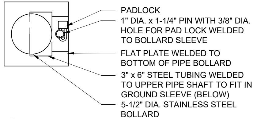
BOLLARD - REMOVABLE: PLAN
