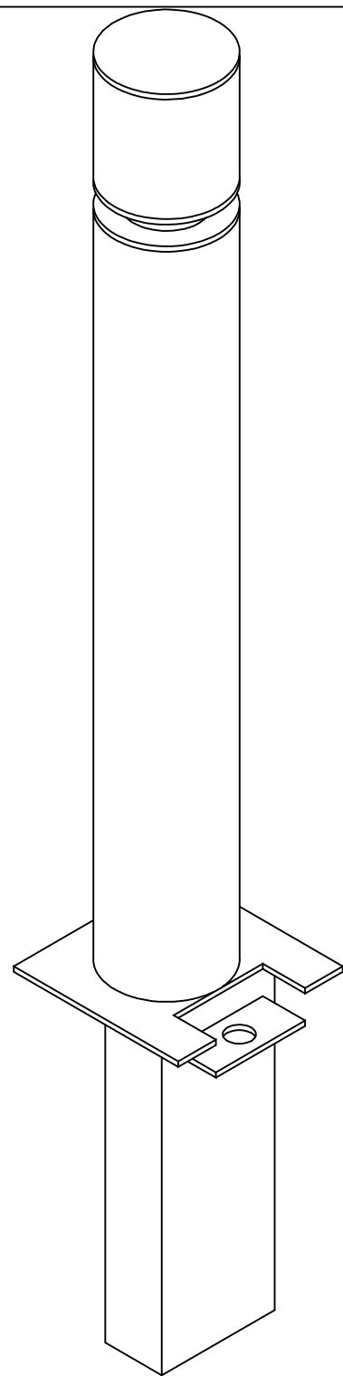
PAINTED BOLLARD - REMOVABLE: ISOMETRIC SCALE: 1-1/2"=1'-0"
